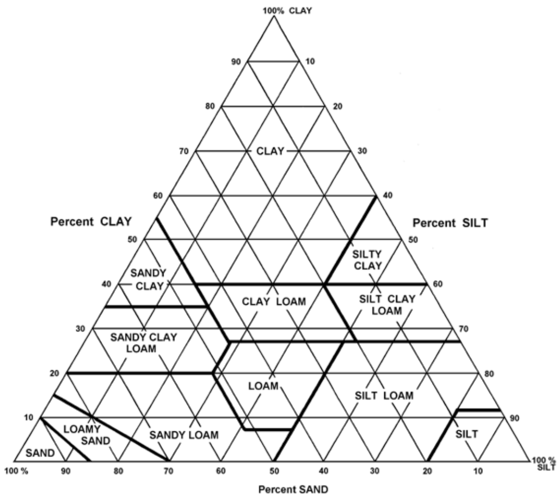
Soil Texture Triangle
